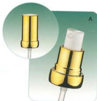
AGR 3010004(A/L) Specification: \Phi 16/410 Discharge Rate: 0.20 \pm 0.02 \text{ ml/T}
