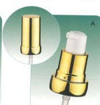
AGR 3010005(A/L) Specification: \Phi 16/410 Discharge Rate: 0.20 \pm 0.02 \text{ ml/T}
