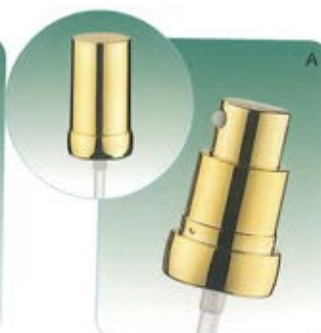
AGR 3010003(A/L) Specification: \Phi 18/410 Discharge Rate: 0.20 \pm 0.02 \text{ ml/T}
